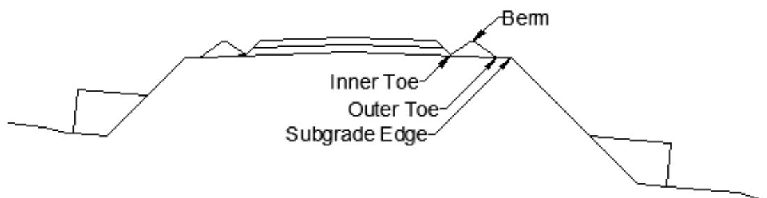
Cross Section
